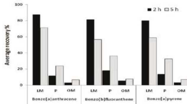
Fig. 3. Average recovery (n = 3) of PAH found in the three different parts of the culture (liquid medium (LM), protozoa (P) and insoluble organic matter (OM)) at two exposure times.
