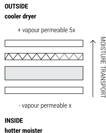
Figure 6: Recommended moisture management in cool climates.
