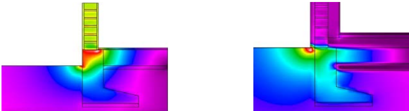
Figure 11: Heat flow through materials in traditional and improved wall / foundation building junction
