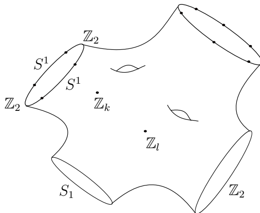
FIGURE 1. Example of an orbit space of an isometric circle action on a closed Alexandrov 3-space.
