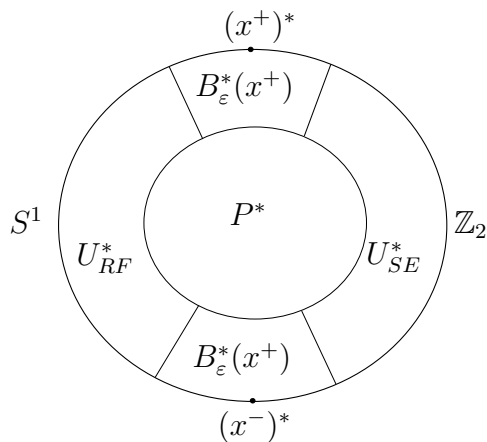
FIGURE 2. Decomposition of X^* into neighborhoods with cross-sections.
